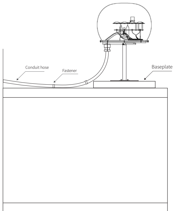
Method②: Install on the balcony
